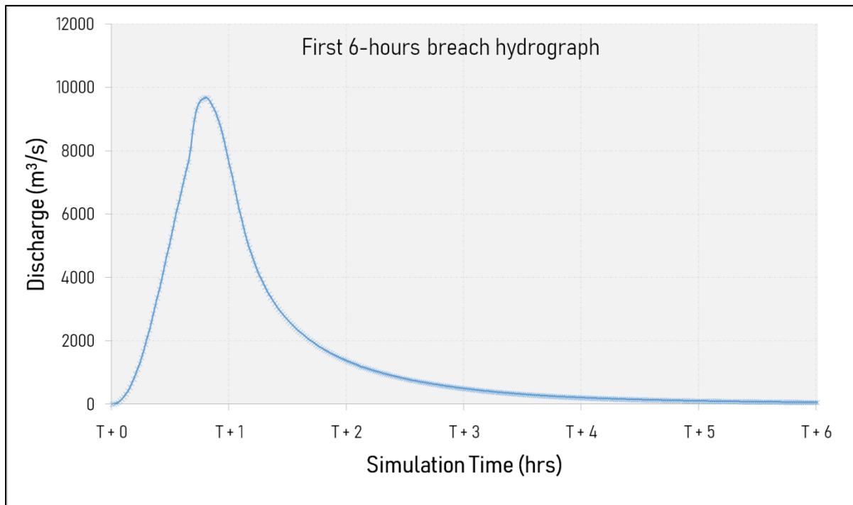
Figure 22: GLOF hydrograph for Scenario-2 (100% volume discharge - Piping failure)
