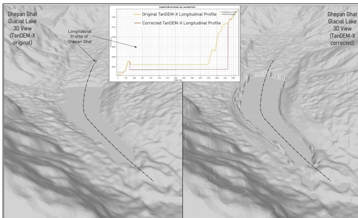
Figure 12: Reconditioned TanDEM-X DTM of Ghepan Ghat Lake
