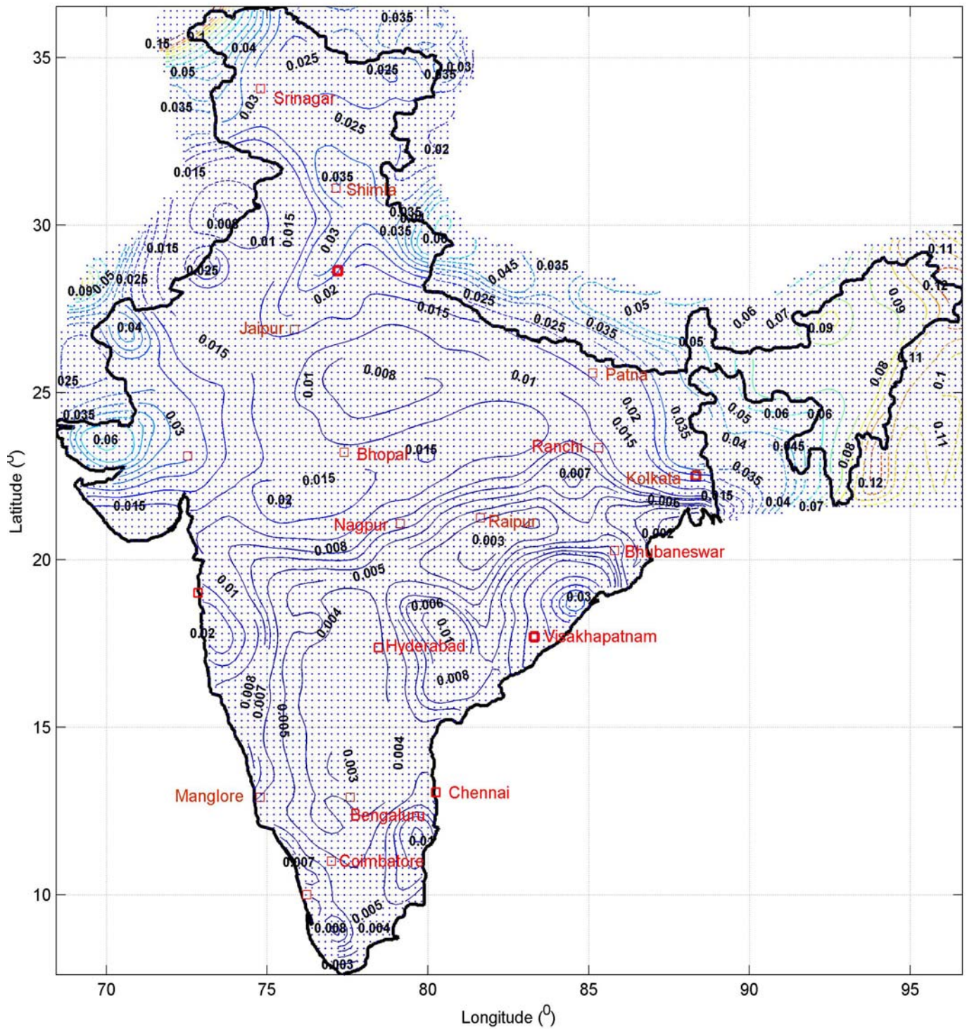
Fig. 5.10 Spectral Acceleration at T = 1.25 sec and 5% damping with 10% probability of exceedence in 50 years (Return Period ~500 years) on A-type Sites
