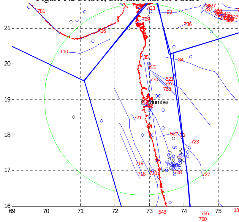
Fig 5.3. Seismic influence zone for Mumbai. Blue lines indicate the boundaries of different source zones
