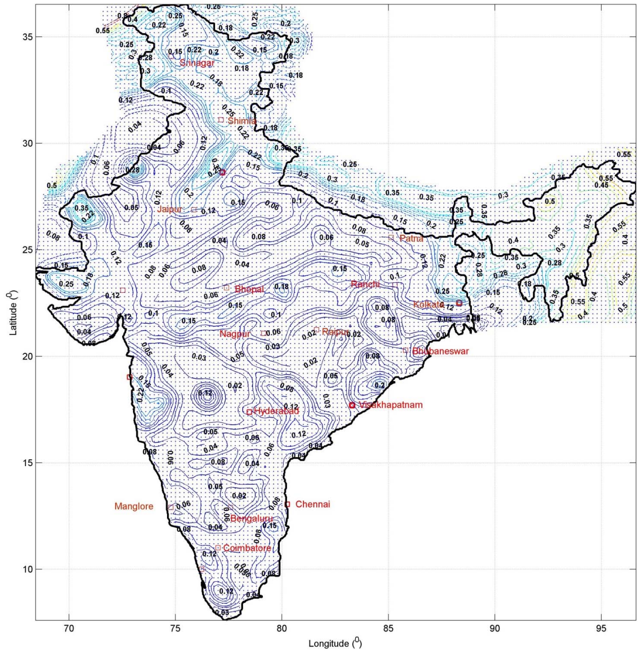
Fig 5.5 PGA Contours with 2% probability of exceedence in 50 years (Return Period ~2500 years) on A-type Sites
