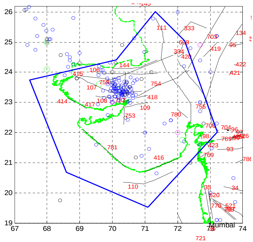
Figure 5.1 Faults and epicenters in source zone 27
