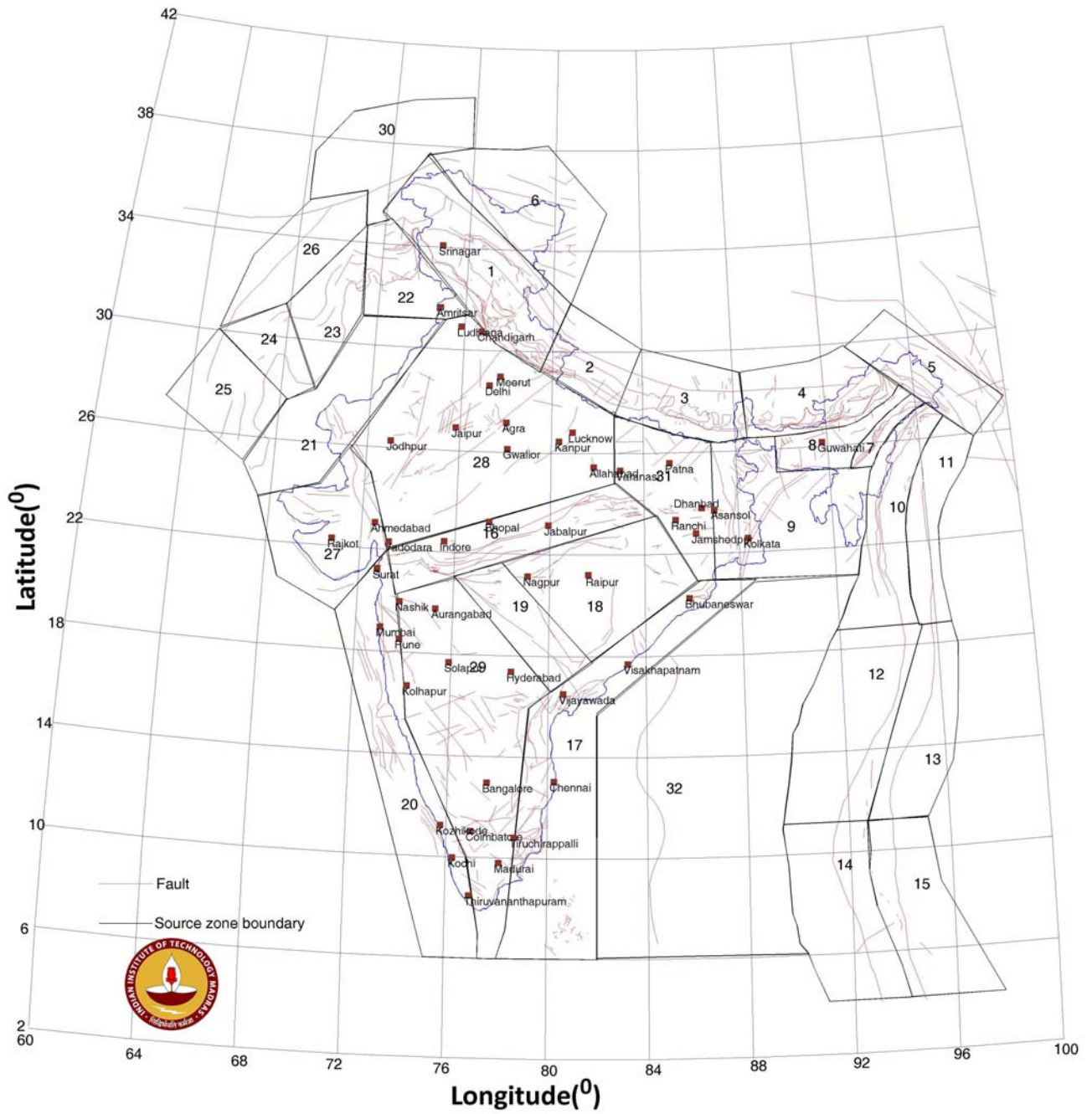
Figure 2.3 Thirty-two Seismogenic Zones of India
