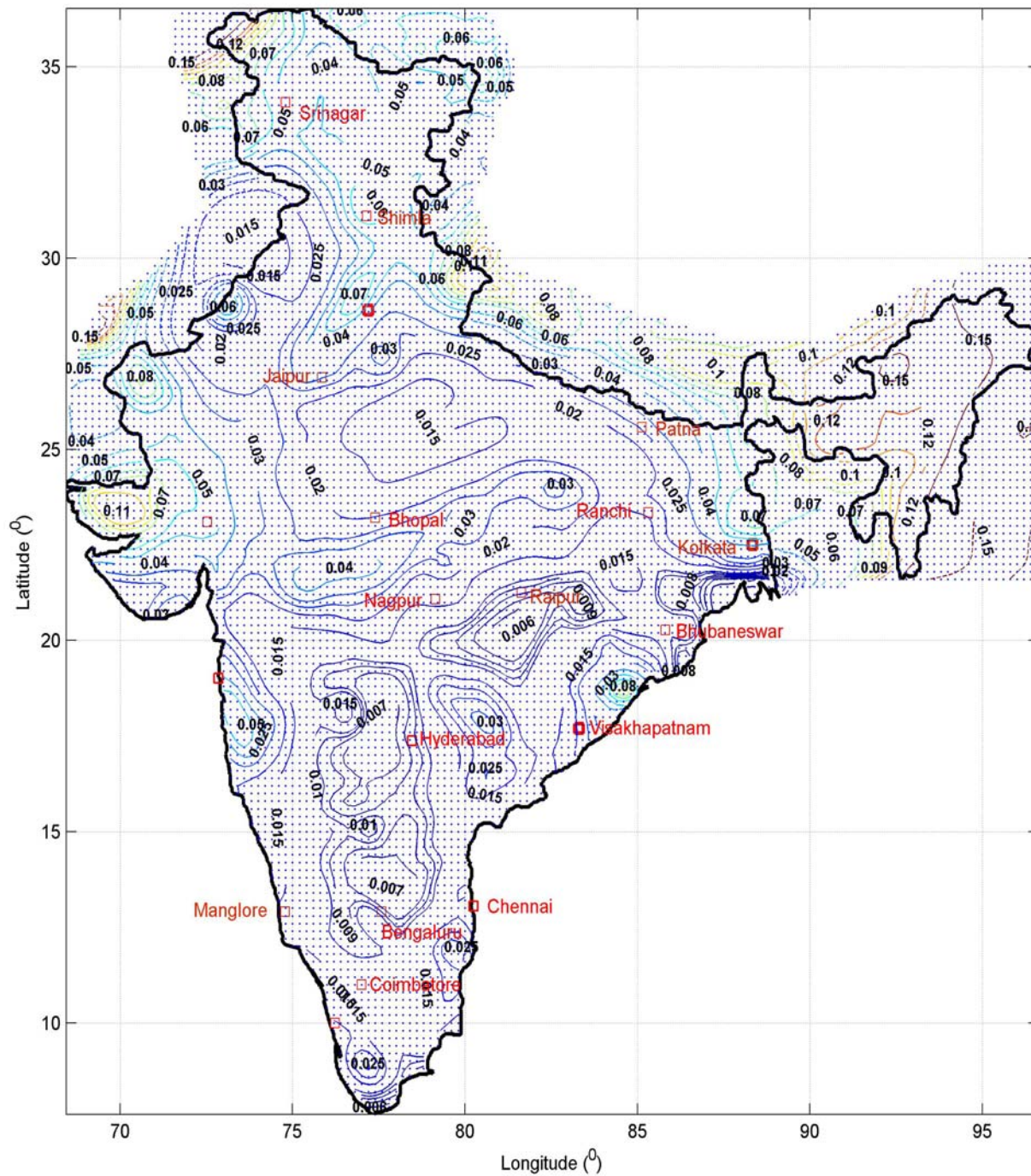
Fig. 5.8 Spectral Acceleration at T=0.5\text{sec} and 5% damping with 10% probability of Exceedence in 50 years (Return Period \sim 500 years) on A-type sites
