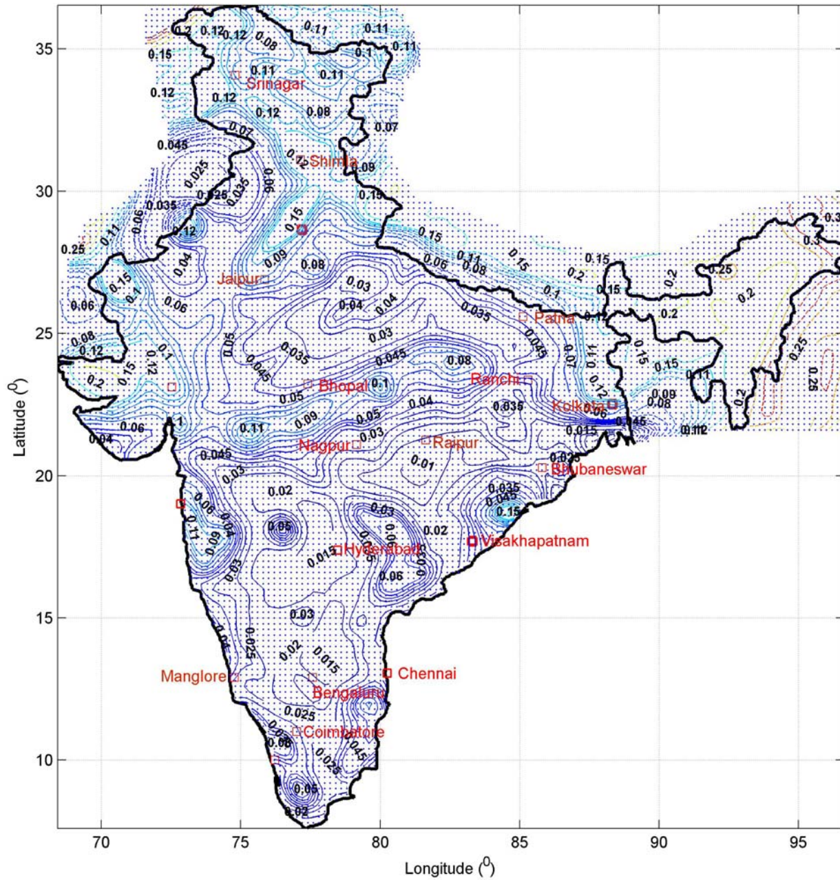
Fig. 5.9 Spectral Acceleration at T=0.5\text{sec} and 5% damping with 2% probability of exceedence in 50 years (Return Period ~2500 years) on A-type sites
